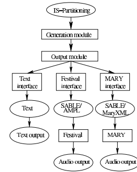
Figure 4: GoDiS-TTS Interfaces
