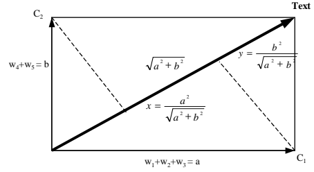
Figure 3: Vector space property
