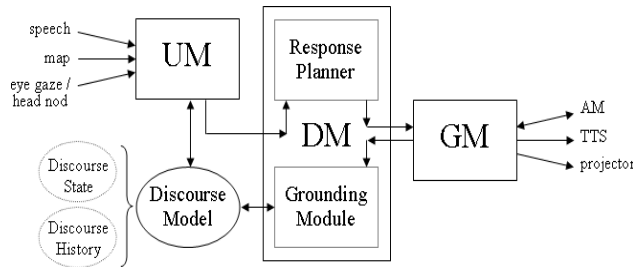
Figure 3: MACK system architecture
