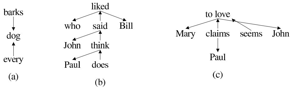
FIG. 7 – Derivation trees
