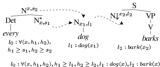
FIG. 3 – Quantifiers
