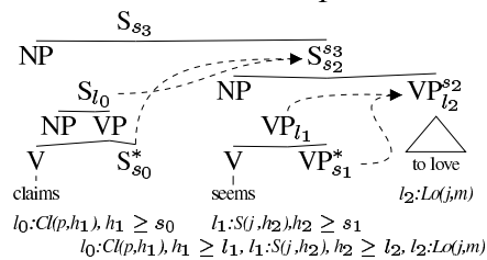
FIG. 9 – Raising verbs
