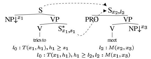
FIG. 6 – Control verbs
