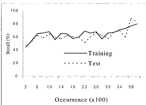
Figure 4: Recall-Occurrence Relationship
