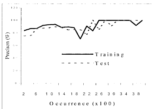
Figure 3: Precision-Occurrence Relationship
